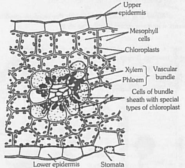
Fig : 4.3-7 Cross section of leaf showing "kranz" type of anatomy
