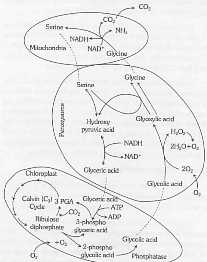
Fig : 4.3-10 The biochemical pathway of photorespiration
