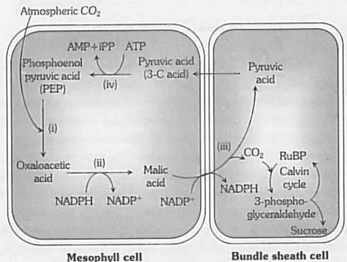
Fig : 4.3-8 Hatch-slack's pathway (cycle) Enzyme : (i) Phosphoenol pyruvate carboxylase, (ii) Malate dehydrogenase, (iii) Decarboxylase, (iv) Pyruvate orthophosphate dikinase
